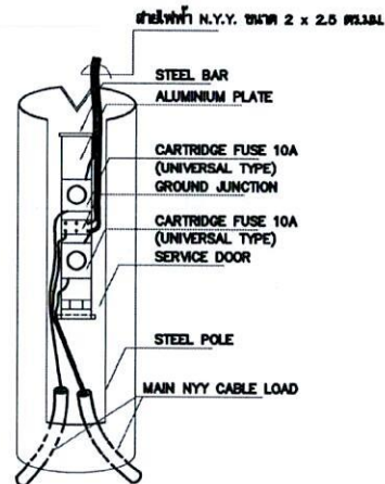
PULL OUT ELECTRICAL CONNECTION
