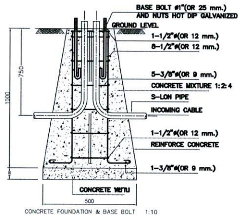
CONCRETE FOUNDATION & BASE BOLT 1:10
